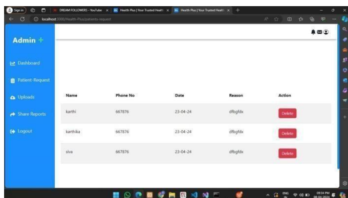
Figure 3.6 Patient Record
