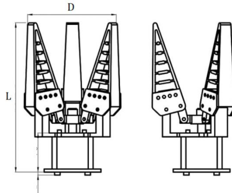
Figure 5: Three Finger Gripping End Effector
