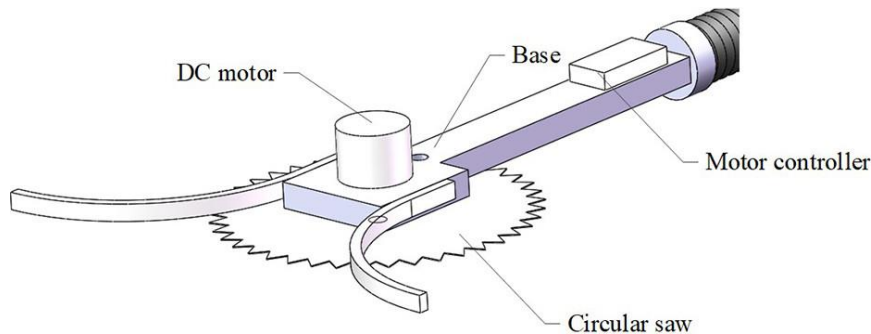
Figure 6: Single Blade Pruning Cutter End Effector
