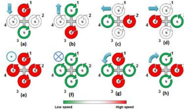
Figure 4 : Basic Flight Movements Of A Quadcopter [10]
